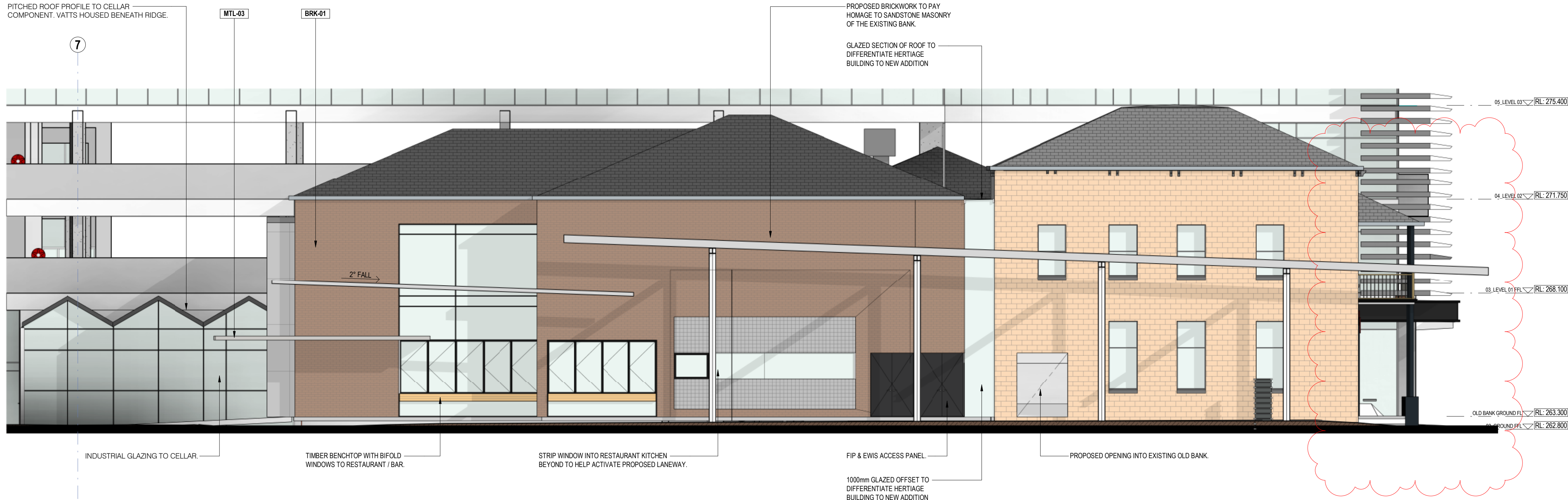
(1) PROPOSED NORTH EAST ELEVATION (LANEWAY) 1 : 100
